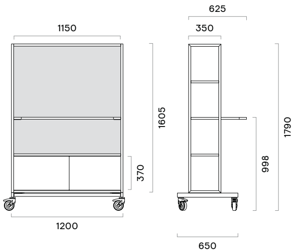
Mobile workstation with fixed cabinet and back panel
